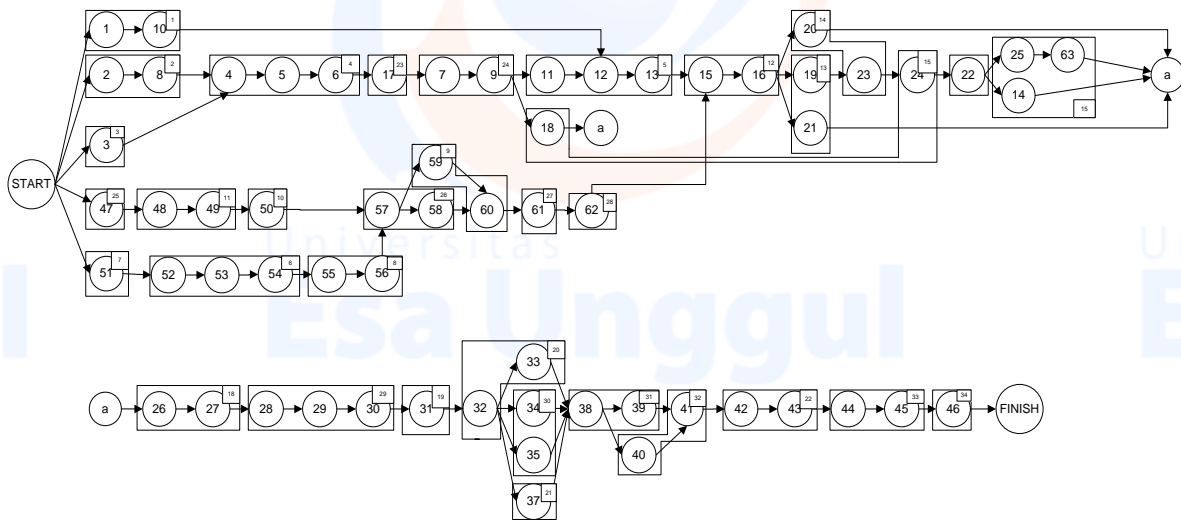
Figure 2. Precedence Diagram of XYZ, Co.'s Line 1
