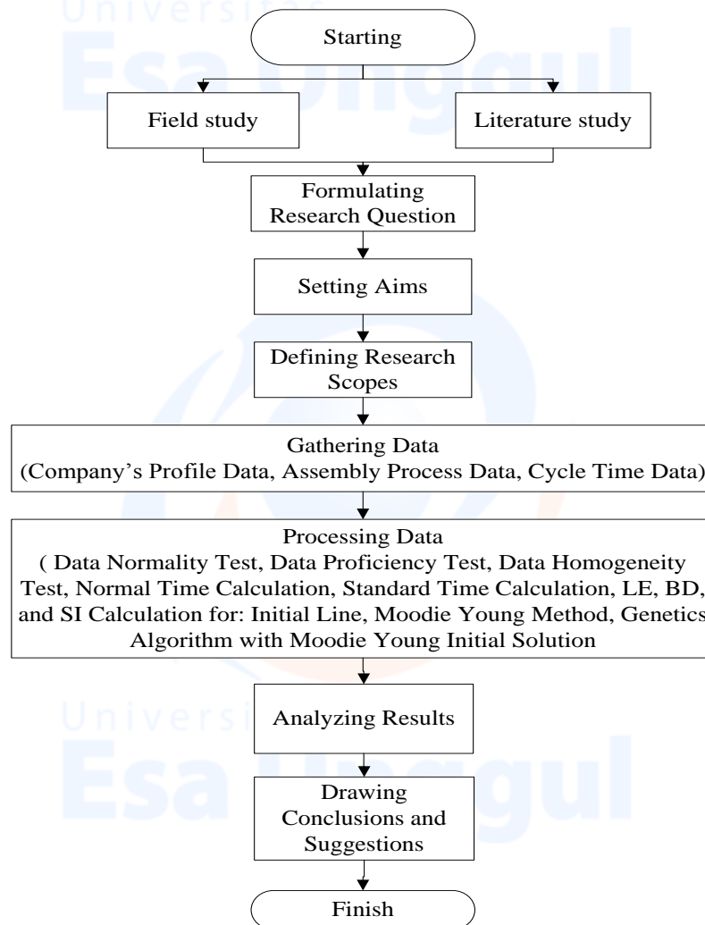
Figure 1. Research Flowchart
