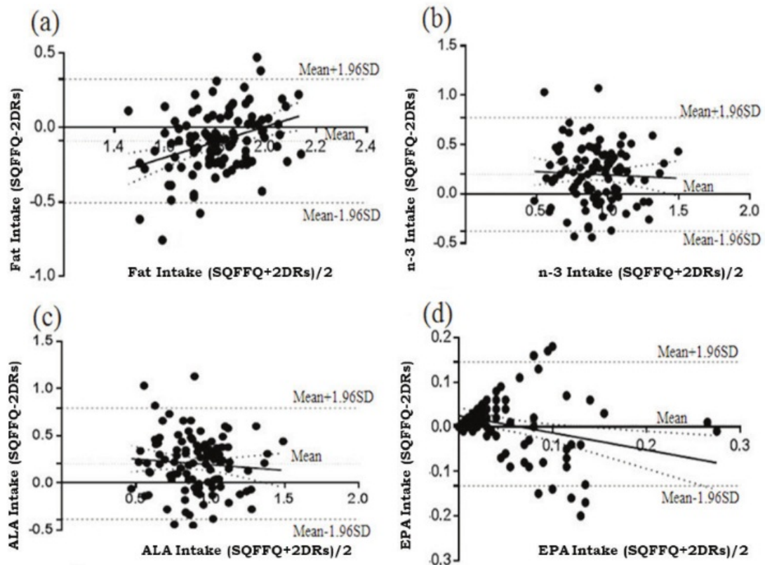
Figure 4. Bland–Altman plot showing agreement between the average of SQ-FFQ and the 2DRs in estimating the intakes of (a) fat, (b) n-3, (c) ALA, alpha linolenic acid and (d) EPA, eicosapentaenoic acid. After natural log transformation. SQ-FFQ = semi-quantitative food frequency questionnaires; 2DRs = two-day 24-hour dietary recalls
