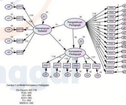
Fig. 2. The Goodness of Fit (GOF) Model
