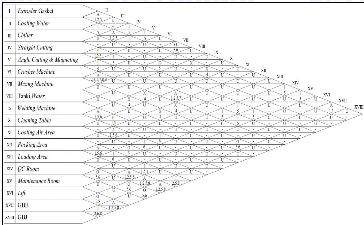
Gambar 2. Activity Relationship Chart(ARC) LiniProduksi Gasket PT.Z
