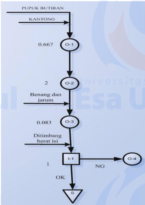
Gambar 2 Operation Process Chart Unit Pengantongan Pupuk Urea
