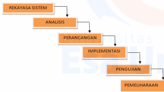
Gambar 2 Metode Waterfall
