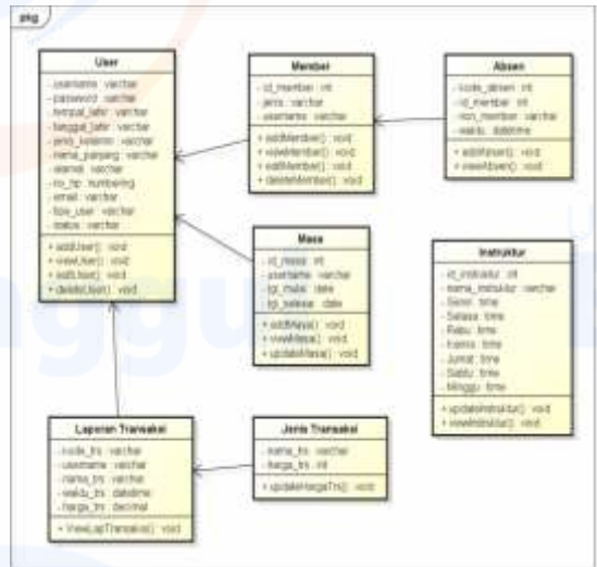
Gambar 5. Class diagram Analisis Sistem
