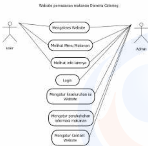
Gambar. 6 Use Case Diagram
