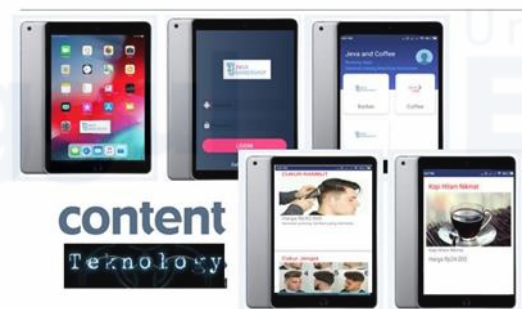
Figure 1. Online Registration
