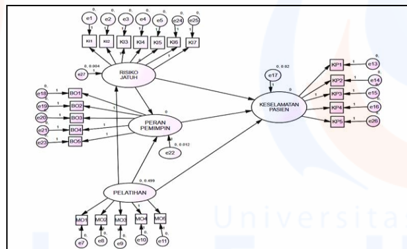
Gambar 4. 1 Model Confirmatory Factor Analysis
