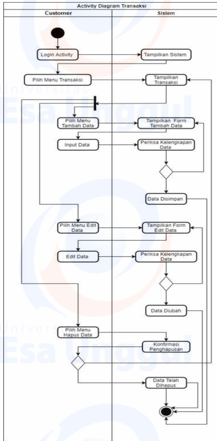
Gambar 6 Activity Diagram Transaksi
