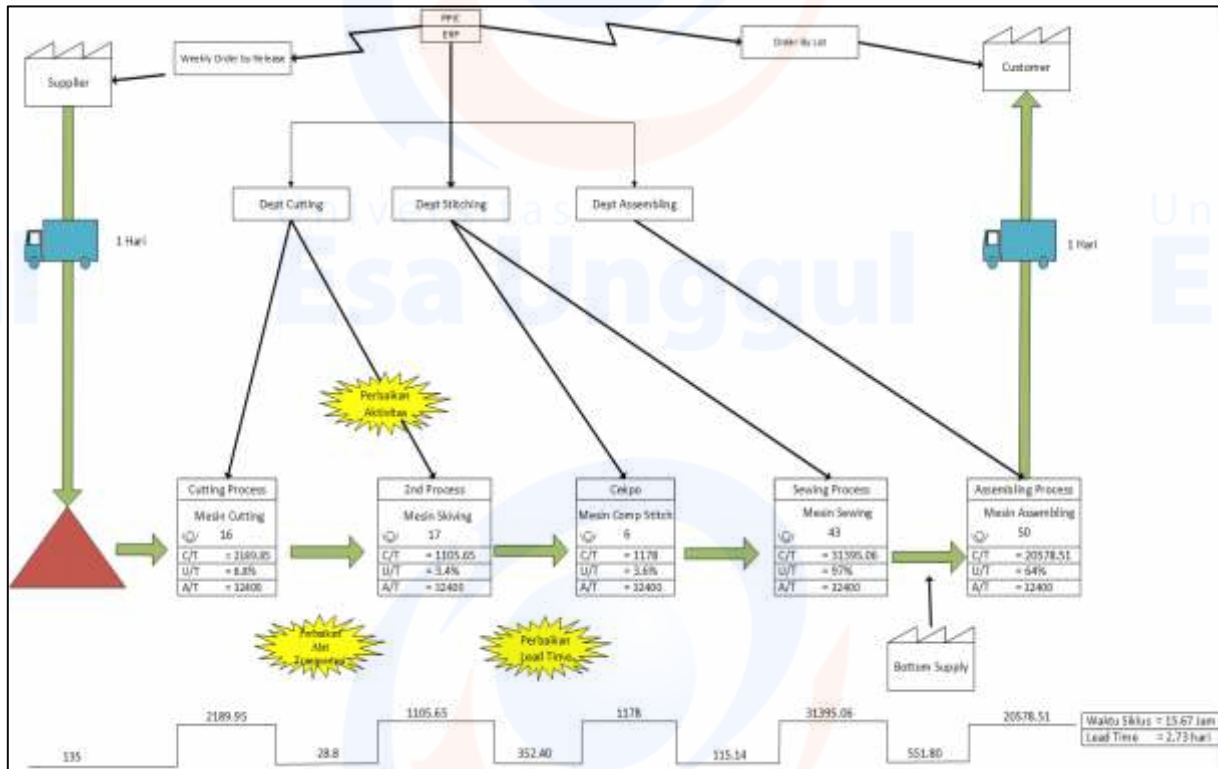
Gambar 6 Future Stream Mapping
