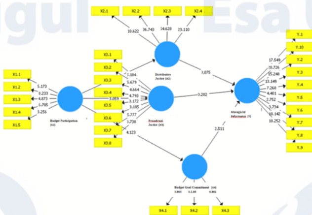
Figure 3. PLS model
