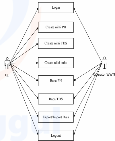
Gambar 9 Use Case Diagram
