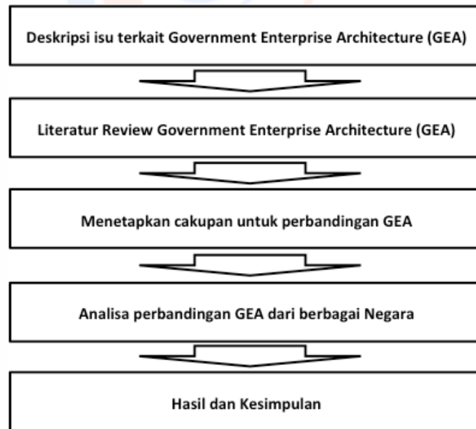
Gambar 3. Metode Penelitian
