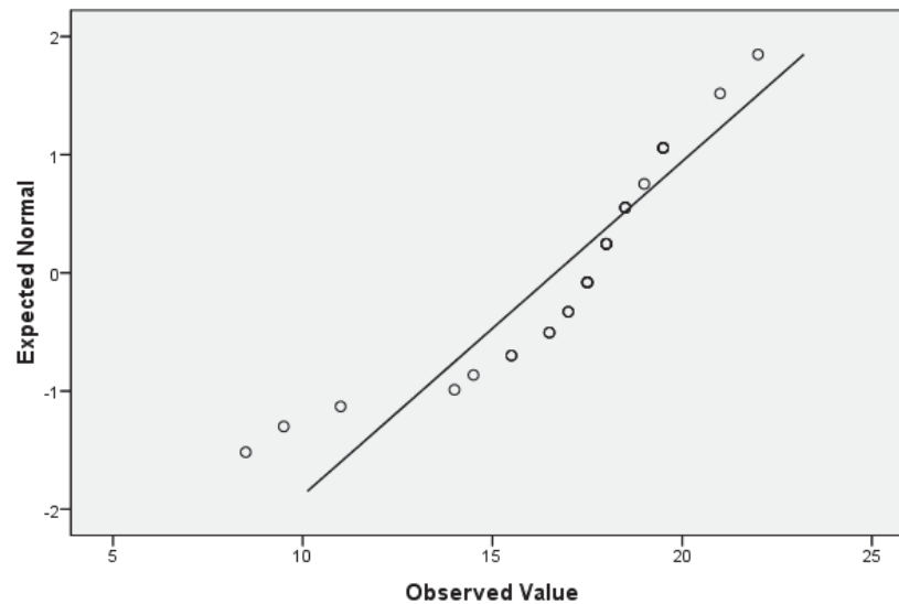
Normal Q-Q Plot of single
