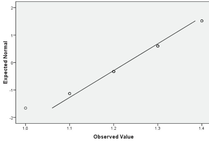
Normal Q-Q Plot of Proporsi
