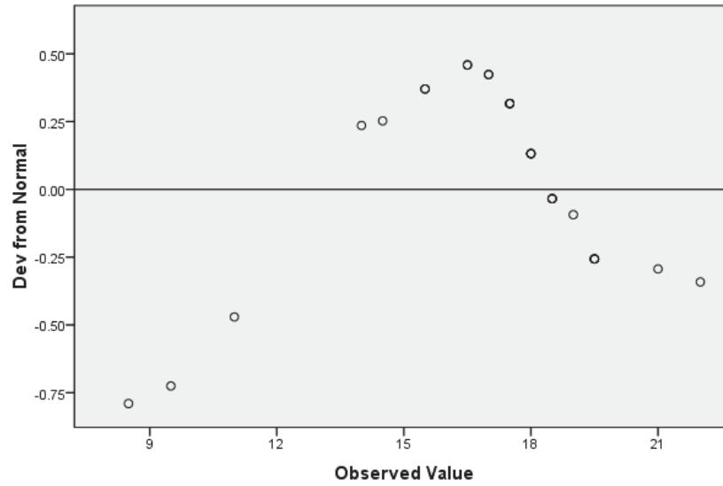
Detrended Normal Q-Q Plot of single
