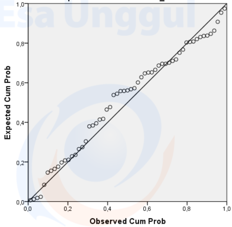
Normal P-P Plot of Regression Standardized Residual Dependent Variable: ROE_1
