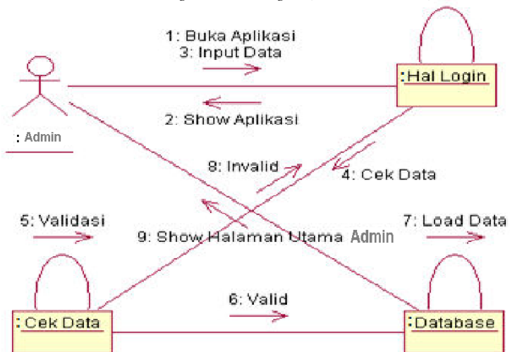
Collaboration Diagram Admin Login. (Sumber : Penulis)
