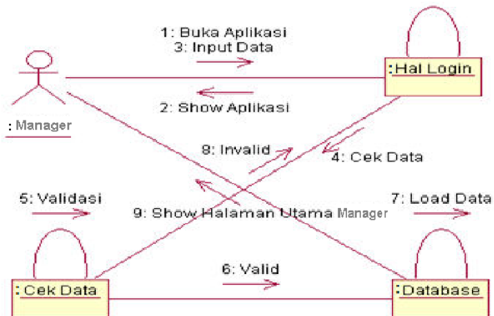
Collaboration Diagram Manager Login. (Sumber : Penulis)
