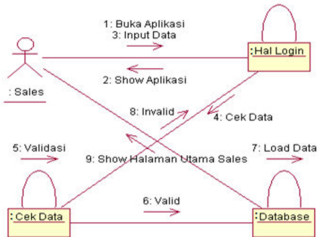
Collaboration Diagram Sales Login. (Sumber : Penulis)
