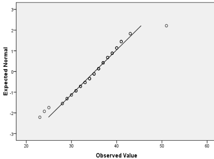
Normal Q-Q Plot of Motivator
