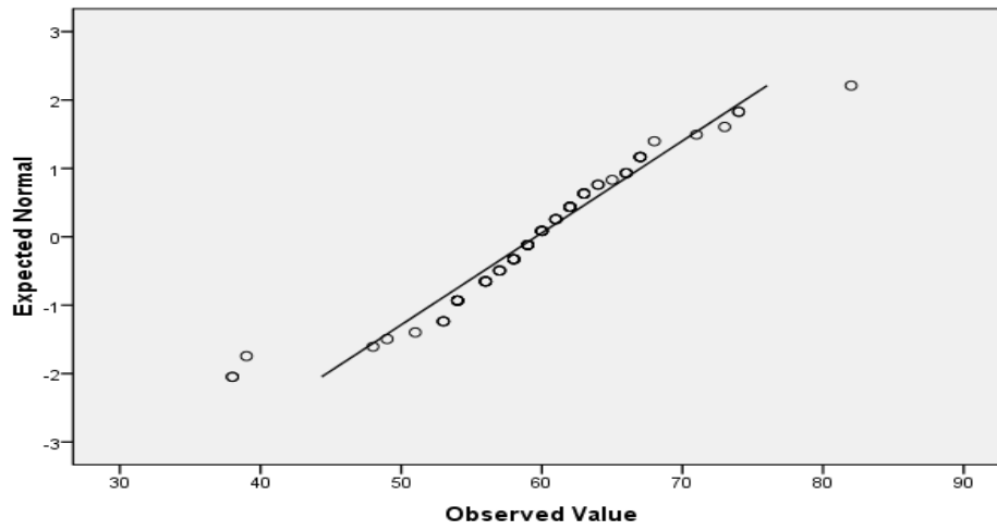
Normal Q-Q Plot of Hygiene
