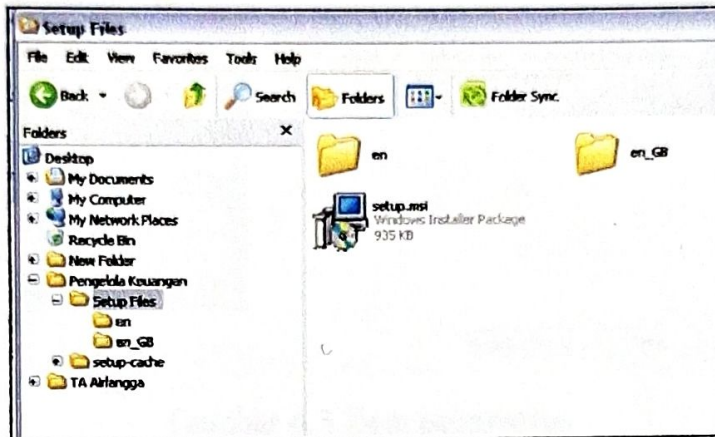
Gambar 4.1 Setup.msi
