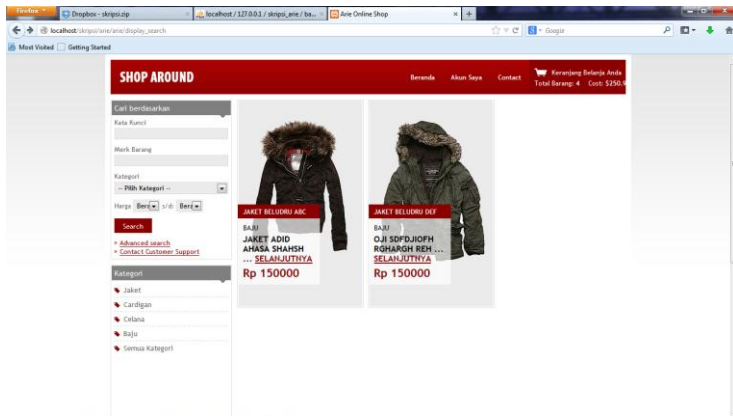
Gambar Layout Search
