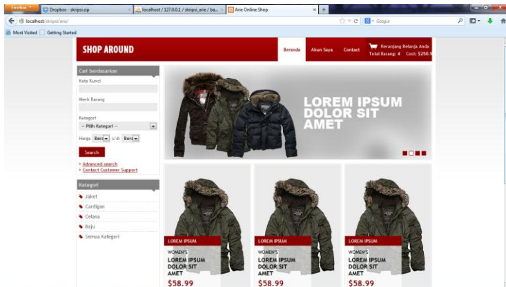
Gambar Layout beranda
