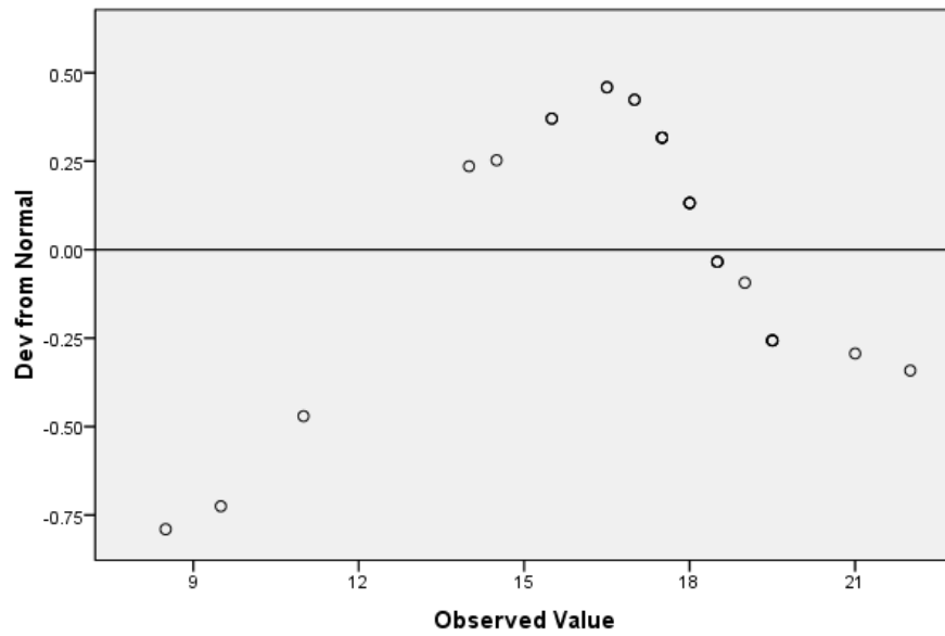
Detrended Normal Q-Q Plot of single
