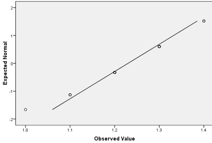
Normal Q-Q Plot of Proporsi
