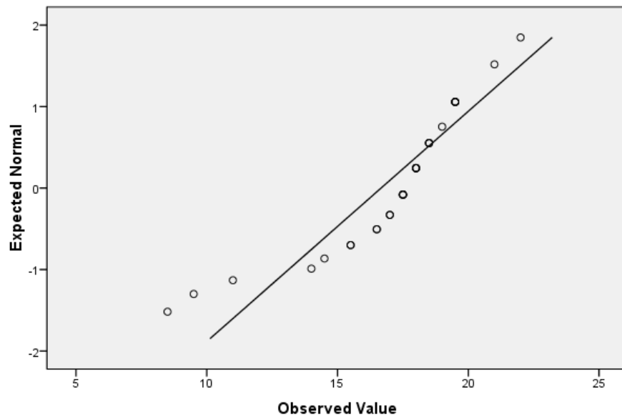
Normal Q-Q Plot of single
