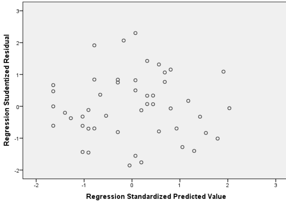
Scatterplot
