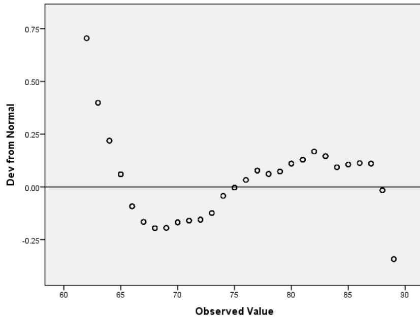
Detrended Normal Q-Q Plot of STRES KERJA
