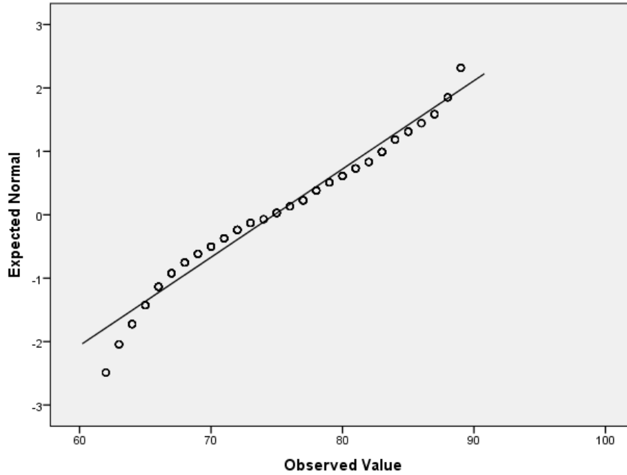
Normal Q-Q Plot of STRES KERJA
